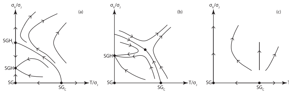
FIG. 7. Schematics of possible renormalization flow scenarios for the variances of the coupling constants, \sigma_J , and magnetic fields, \sigma_h , of a spin-glass model in d < d_u . Note that even if the RG scheme starts with a uniform external field, a random field emerges after a few iterations. 138 The points SG, SGH, SG_c , and SGH_c denote the fixed points (FPs) associated with the spin-glass phase, the spin-glass phase in a field, the critical point for spin glasses without field, and the critical point for spin glasses in a field, respectively. (a) In this scenario, the transition in a field is present and its associated FP lies at T = 0 , i.e., the couplings and the fields become much larger than the temperature under RG. 138 (b) In this scenario, the transition in a field is present and the associated FP is standard, although nonperturbative. 139 (c) In this scenario, there is no FP in a field and, hence, no transition. 140,141
