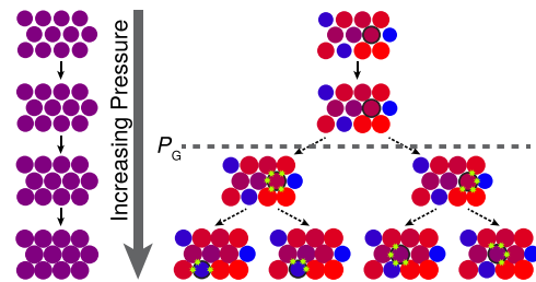
FIG. 6. Schematic illustration of a Gardner-like scenario for polydisperse crystals. A perfect crystal (purple particles) has only one well-separated densest packing. A crystal of polydisperse particles (colored from red to purple, according to their growing particle radius), by contrast, has a large number of nearly equivalent packings. Beyond the pressure onset of Gardner-like physics, at P_G , such systems are forced into irreversible constraints. For the sake of illustration, consider the particle outlined in black. It is free to collide with all its nearest neighbors at low pressures, but forced to have one or another set of collisional contacts (green stars) as pressure increases. This overall process is cooperative and thus cannot be reduced to such a simple local description, but this illustration can nonetheless be useful to understand and explain the physics at play. Reprinted with permission from P. Charbonneau, E. I. Corwin, L. Fu, G. Tsekis, and M. van der Naald, Phys. Rev. E 99 , 020901(R) (2019). Copyright 2019 American Physical Society.
