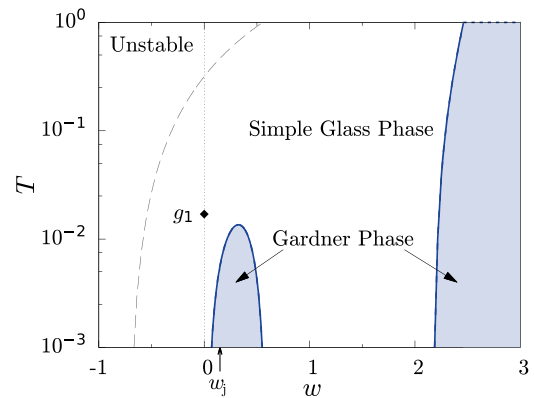
FIG. 4. Mean-field phase diagram for soft repulsive WCA particles. The glass at point g_1 is prepared under equilibrium conditions at temperature T_{g_1} and density \rho_{g_1} and is then adiabatically followed up to different temperatures and densities, measured as w = \ln[\rho/\rho_{g_1}] . The glass state then either fluidizes (unstable region, beyond the dashed line), remains within an ergodic cluster (simple glass phase), or undergoes a Gardner transition (dark blue lines) to enter the Gardner phase (light blue areas). This example illustrates that in d \rightarrow \infty soft glasses can generically undergo a Gardner transition under a variety of physical conditions, including around the jamming point w_j of the glass prepared at g_1 . Reprinted with permission from C. Scalliet, L. Berthier, and F. Zamponi, Phys. Rev. E 99 , 012107 (2019). Copyright 2019 American Physical Society.
