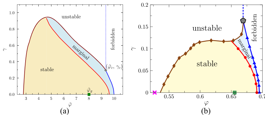
FIG. 5. (a) Theoretical shearing phase diagram of d \rightarrow \infty hard spheres prepared in an equilibrium glass state at scaled packing fraction \hat{\varphi}_g = 8 . Reprinted with permission from P. Urbani and F. Zamponi, Phys. Rev. Lett. 118 , 038001 (2017). Copyright 2017 by the American Physical Society. The glass is first compressed at scaled packing fraction \hat{\varphi} and then strained at shear strain \gamma , resulting in a (\hat{\varphi}, \gamma) stability map. The simple glass (stable) phase is delimited by the yielding (brown) line at lower density and by the shear jamming (blue) line at higher density. A Gardner transition (red) line delimits the Gardner (marginal) phase at high (\hat{\varphi}, \gamma) . (b) Corresponding numerical phase diagram of d = 3 hard spheres prepared in equilibrium at \varphi_g = 0.655 . Adapted from Y. Jin, P. Urbani, F. Zamponi, and H. Yoshino, Sci. Adv. 4 , eaat6387 (2018). Copyright 2018 Author(s), licensed under a Creative Commons Attribution 4.0 License. The qualitative agreement between the mean-field prediction and the d = 3 numerical simulations is remarkable, except in the vicinity of the critical point (gray diamond), where the shear jamming and shear yielding lines merge. The qualitative difference might be explained either in the presence of localized plastic excitations in d = 3 systems (in which the role of the Gardner transition has yet to be clarified) or by the different nature of the yielding transition in d = 3 (shear band nucleation vs spinodal instability).
