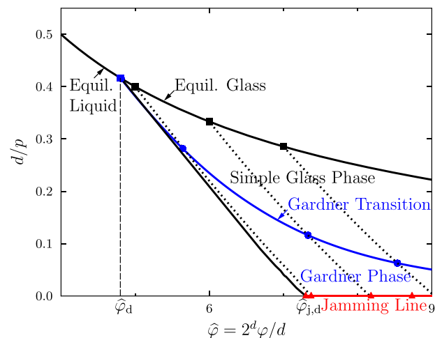
FIG. 3. Phase diagram for hard spheres in the limit d \rightarrow \infty . At equilibrium (solid black line), for \phi < \phi_d the liquid is ergodic, while for \phi > \phi_d a large number of ergodic clusters are separated from one another, which gives rise to equilibrium glass states. Upon slowly compressing any such glass state (dotted lines), a Gardner transition (blue line) is encountered prior to reaching jamming (red line) at infinite (reduced) pressure, p \rightarrow \infty . Republished with permission from P. Charbonneau, J. Kurchan, G. Parisi, P. Urbani, and F. Zamponi, Annu. Rev. Condens. Matter. Phys. 8 , 265-288 (2017). Copyright 2017 Annual Reviews, Inc.
