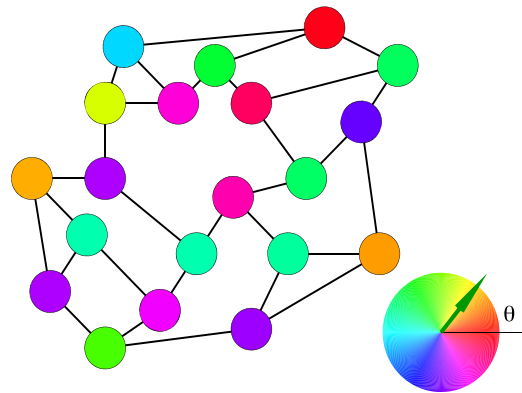
FIG. 9. Illustration of the difference between continuous and discrete variables in the graph coloring CSP. In the standard, discrete setting, q colors are available to color the vertices of a given graph such that no two adjacent vertices have the same color. (In the language of statistical physics, such a solution is the ground state of a Potts antiferromagnet.) In the continuous setting, colors are continuous variables on a circle and can therefore be defined by an angle \theta . The constraint is that the distance between colors on contiguous vertexes should be larger than a given threshold. For any finite graph, in the discrete problem, the set of solutions is discrete and numerable. In the continuous setting, this set is continuous, and its volume goes to zero at a jamming transition. Adapted from H. Yoshino, SciPost Phys. 4 , 040 (2018). Copyright 2018 Author(s), licensed under a Creative Commons Attribution 4.0 License.
