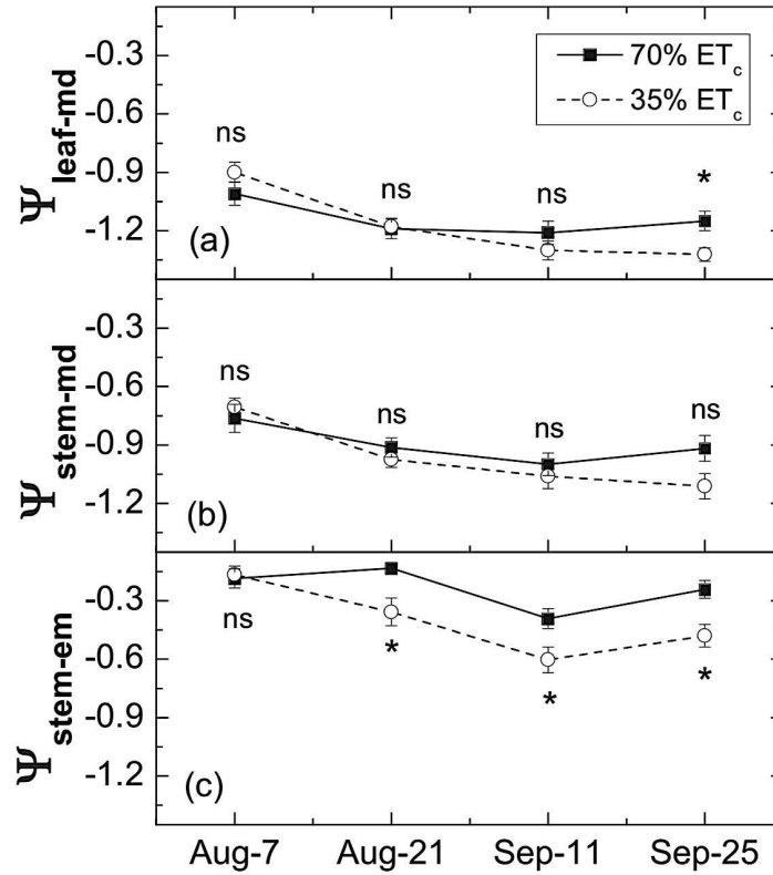
Figure 9 – Seasonal patterns of grapevine water potentials ( \Psi_w ) at two levels of sustained deficit irrigation, 70% of crop evapotranspiration ( ET_c ) and 35% ET_c . Leaf or stem \Psi_w was measured using a leaf pressure chamber at three different times of the day : (a) midday \Psi_{leaf-md} , (b) midday \Psi_{stem-md} and (c) early morning \Psi_{stem-em} . ns and * indicate no significant difference and significant difference at P < 0.05 , respectively. All \Psi_w values reported in units of MPa [Cole, 2015]
