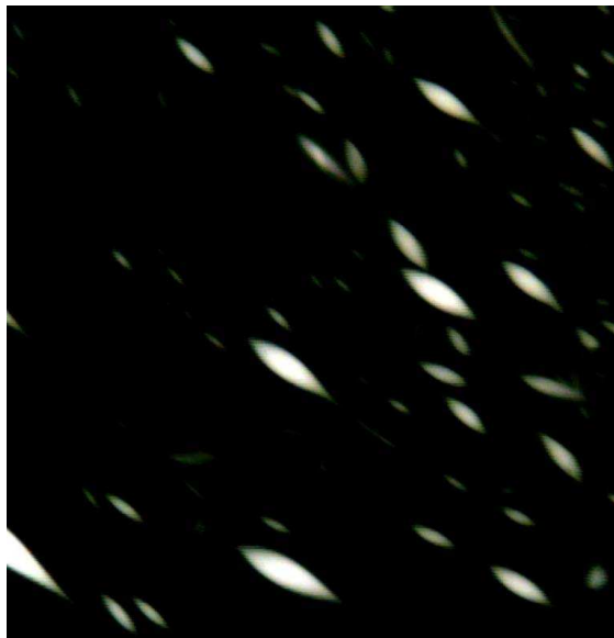
FIG. 2: Polarization microscopic image with crossed polarizers, showing a collection of tactoids in aqueous dispersion of bile-salt stabilized single-wall carbon nanotubes. The image size is 97 \mu\text{m} \times 100 \mu\text{m} .
