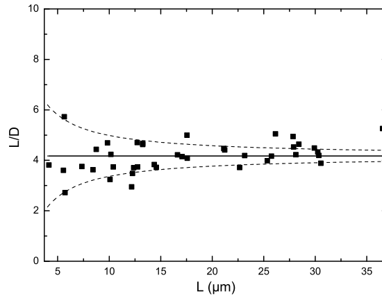
FIG. 4: Aspect ratio of the tactoids versus their length in microns. Full squares: experimental data points. Drawn line: average value deduced from the experiments. Dashed lines: predicted standard deviation presuming that the surface tension is equal to 0.5 nN/m.
